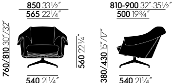
Bascule Lowback, Vierstern-Untergestell
